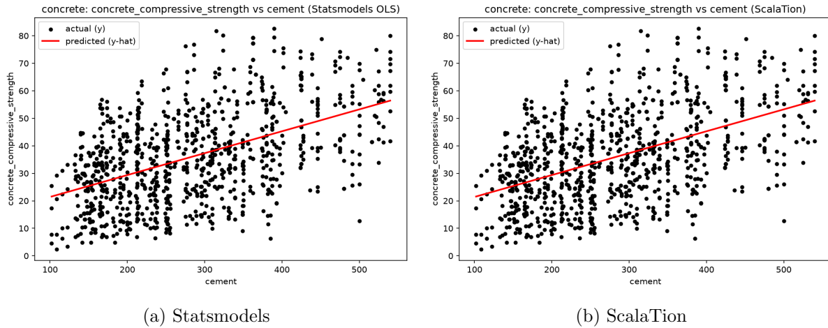
Figure 5: Compressive strength vs. cement content: actual (black) and predicted (red) values.
